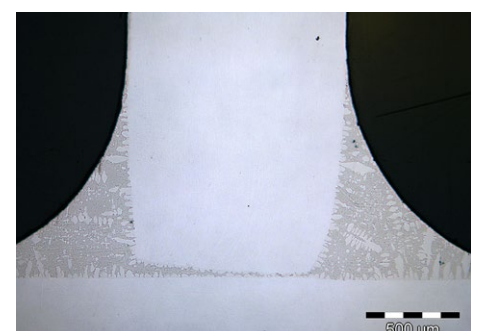
Figure 3. Brazed joint on a T-specimen (Amdry 105)
