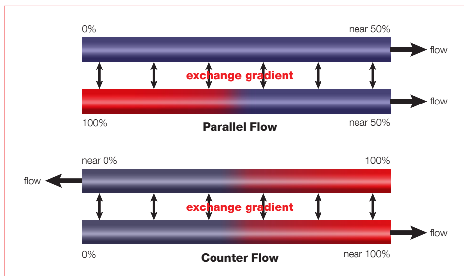
Figure 1. Comparison of parallel flow (top) and counter flow (bottom) heat transfer. Counter flow is much more efficient
