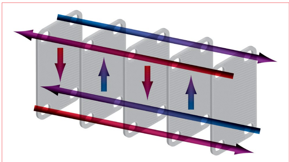
Figure 2. Schematic of a counter flow, plate heat exchanger
